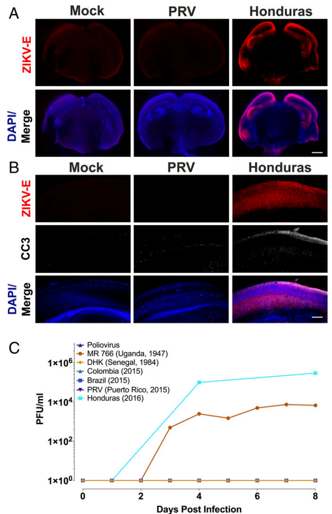
Fig. 5. Replication of two ZIKV isolates in late gestation neural tissue. (A and B) Brain slice cultures from E19 embryos were infected with 10 5 pfu of the indicated ZIKV isolates and at 8 dpi, were fixed and stained with pan-flavivirus antibody against the E glycoprotein (ZIKV-E), cleaved caspase 3 (CC3), and DAPI. Unlike E13 and E15 organotypic slices, E19 slices supported the infection and replication of only the MR766 and Honduran isolates. Staining for ZIKV-E after infection with the Honduran isolate demonstrated viral infection throughout the developing neocortex, with little staining in other brain regions. (Scale bar: 500 and 250 \mu m in A and B.) (C) Time course of replication of multiple isolates of ZIKV in E19 brain slice cultures. Poliovirus, DHK, Colombia, and PRV isolates did not replicate as the lines are superimposed and not readily visible. Results are representative of three independent experiments.
